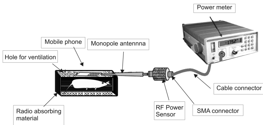
Fig. 1— Calibration methodology of power emitted from mobile phone during exposure.
